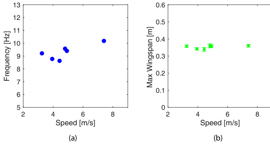
Figure S1: Wing kinematics as a function of speed. (a) Flapping frequency, defined by the up/down motion of the shoulder marker in body-fixed coordinate B . (b) Maximum wingspan is two times the greatest distance between the body sternum marker and the left wingtip. The vertical bar indicates one standard deviation of uncertainty resulting from a Monte Carlo randomization process.
