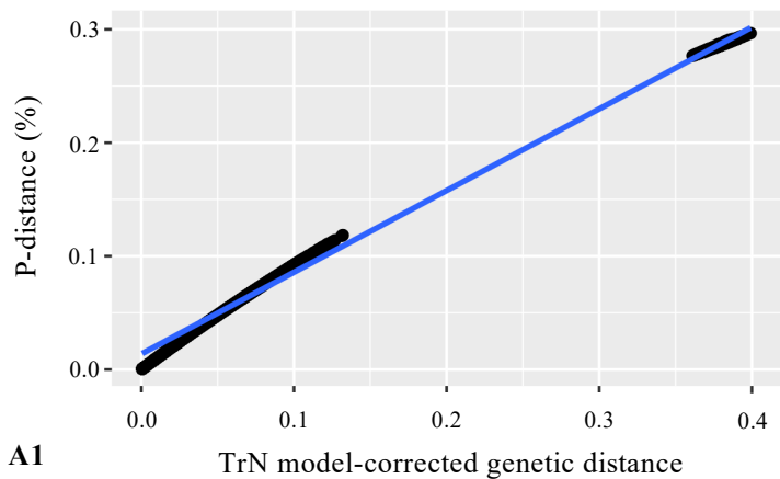
Saturation plot of 1 st positions
