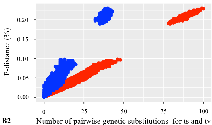
Saturation plot of 2 nd positions
