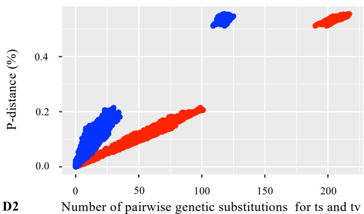
Saturation plot of 3 rd positions
