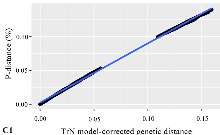
Saturation plot of 2 nd positions
