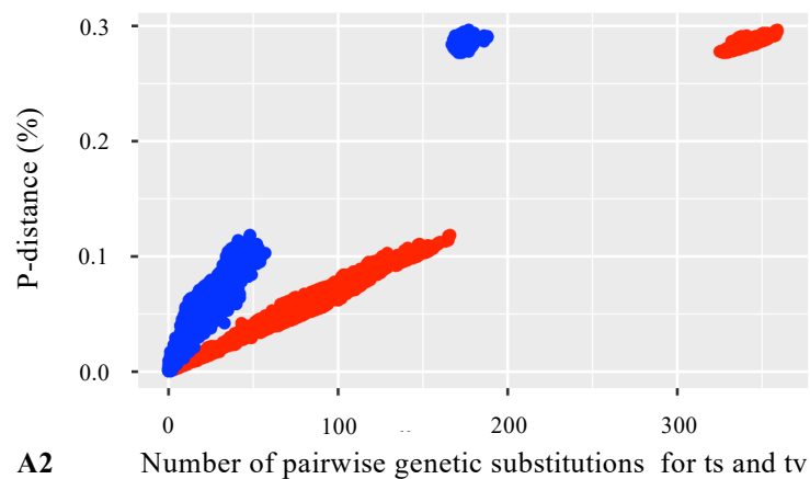
Saturation plot of 1 st positions
