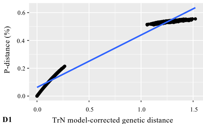
Saturation plot of 3 rd positions
