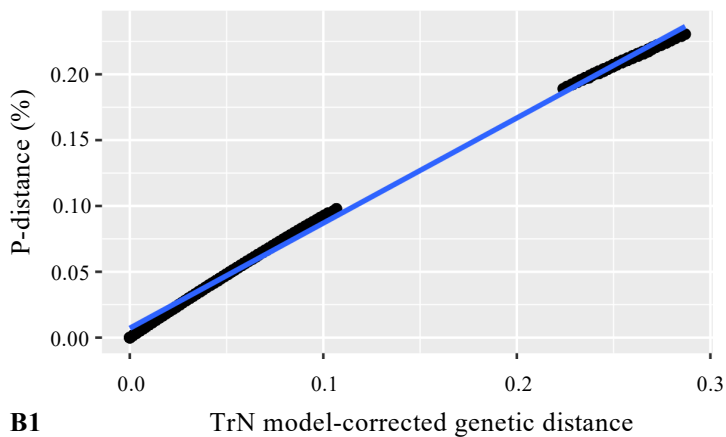
Saturation plot of 2 nd positions
