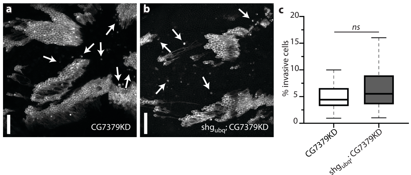
Figure S3: E-cadherin overexpression cannot rescue CG7379KD induced cell delamination
