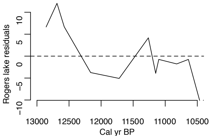
Figure S1. Residuals from the linear model in figure 1c. The long-term trend in residuals indicates autocorrelation that future analyses should account for, either within the covariance matrix of the residuals (e.g. using an autoregressive generalized least squares model) or by evaluating additional environmental covariates that may account for the trend
