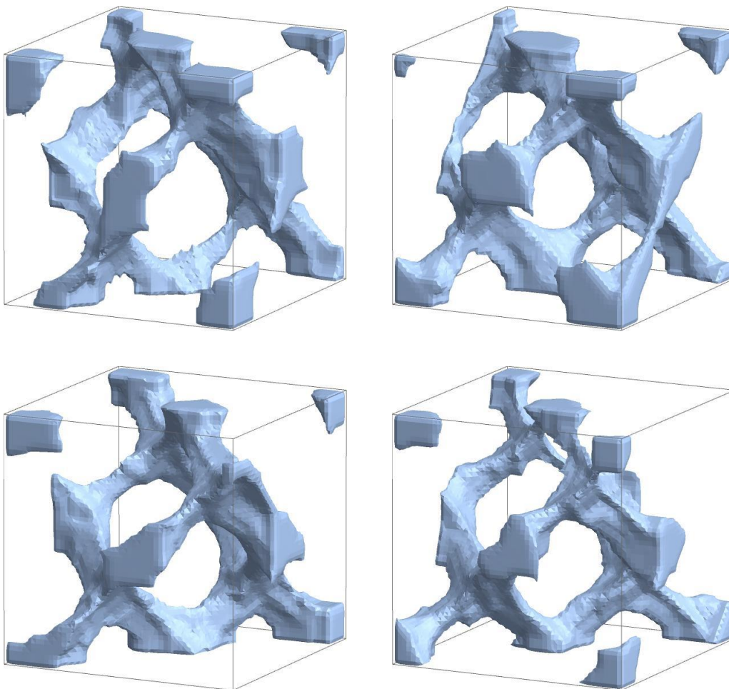
Figure S2 Four examples of the cubic unit cell taken out from the reconstructed 3-dimensional structure. Their positions are shifted by primitive translational vectors from the cell shown in Fig. 7(a).
